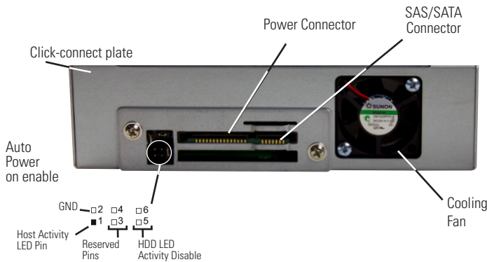
Figure 2: DX115 Receiving Frame Rear Panel
