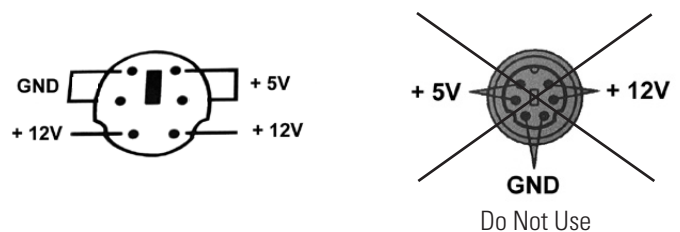
Figure 3: Power Connector
