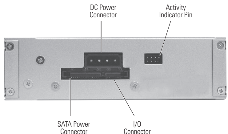
Figure 2: Rear Panel
